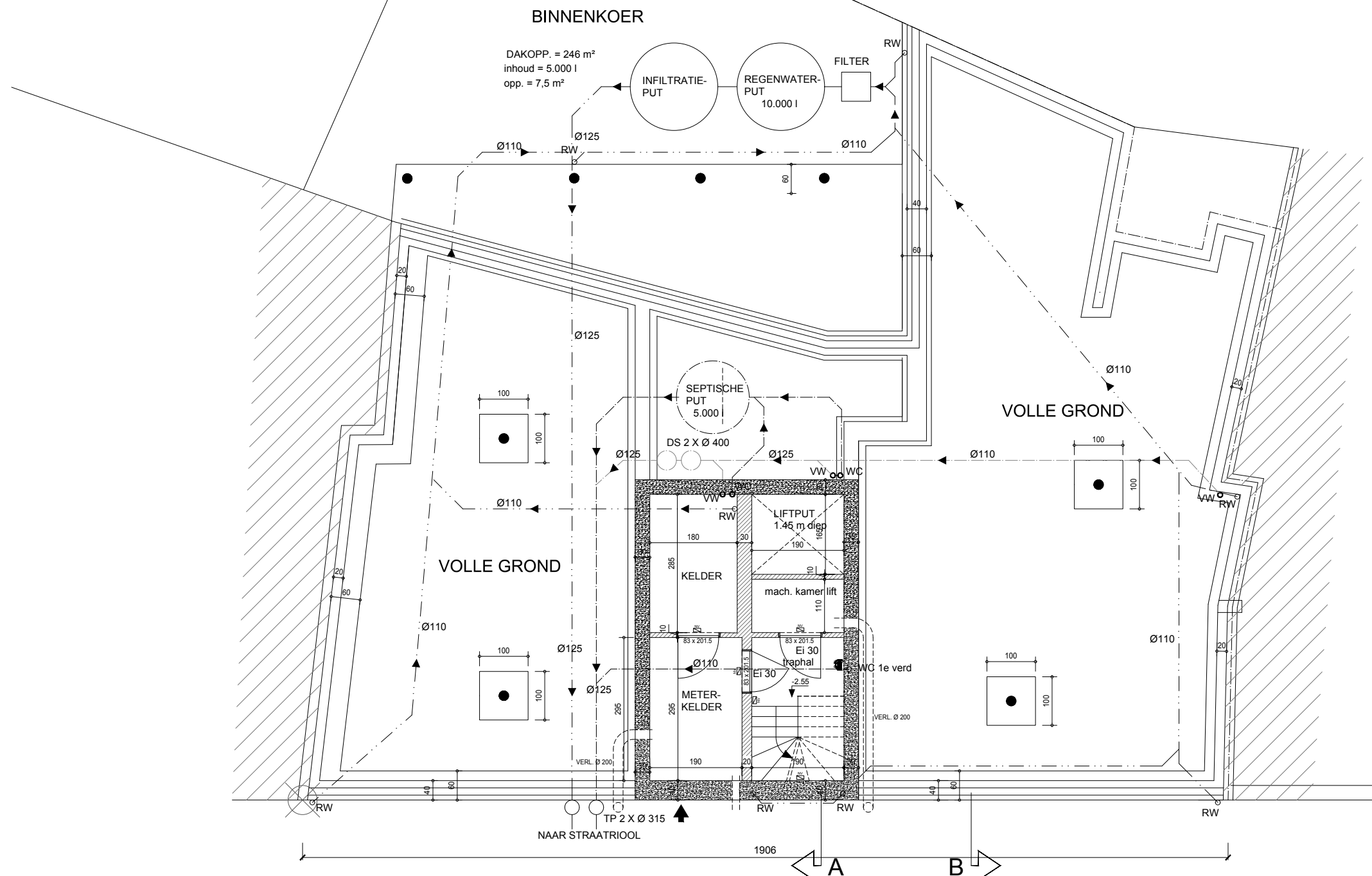
PLAN KELDER + FUNDERING + RIOLERING
