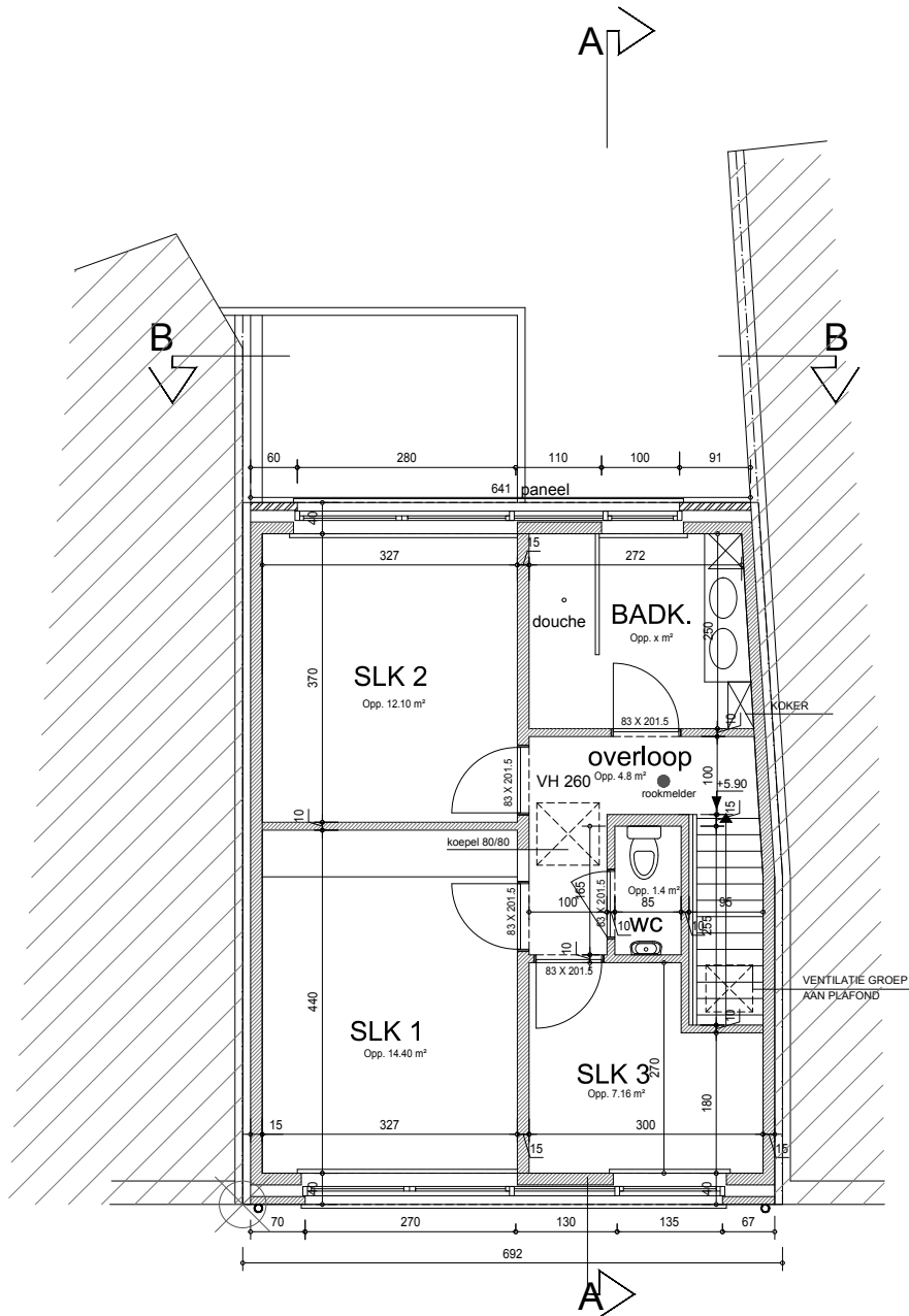
PLAN VERDIEPING 2
