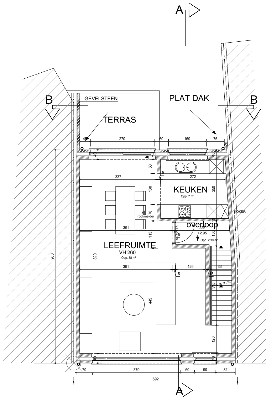
PLAN VERDIEPING 1
