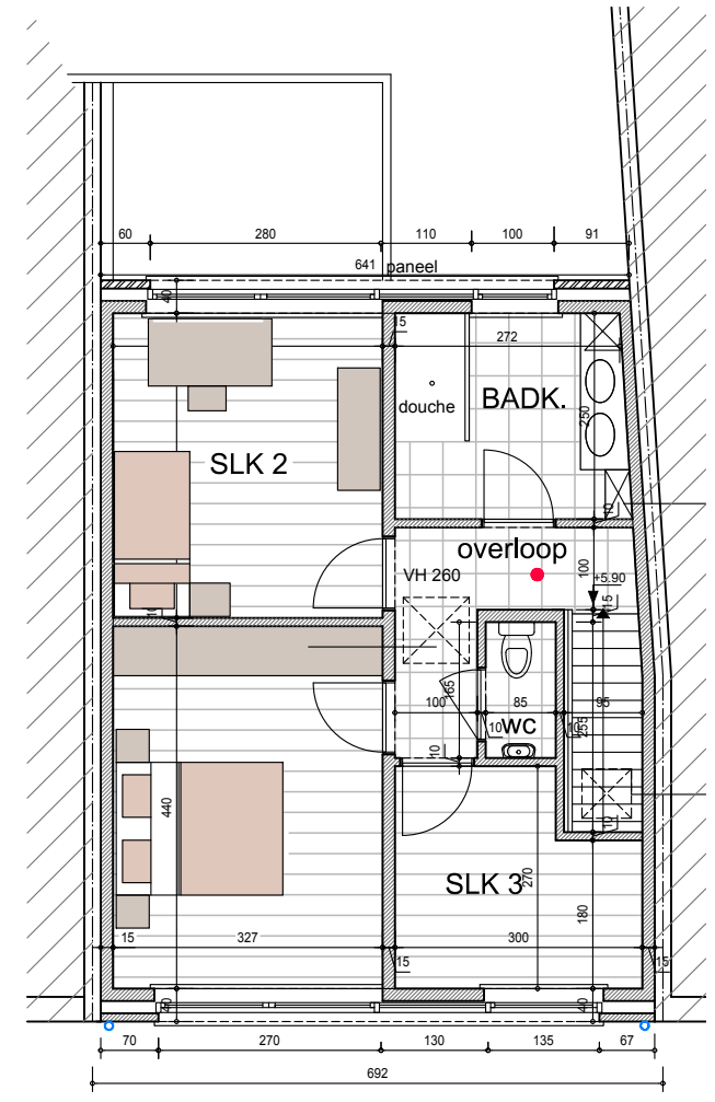
PLAN VERDIEPING 2
