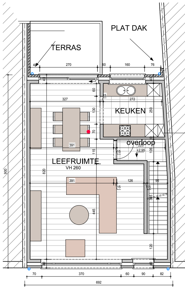
PLAN VERDIEPING 1
